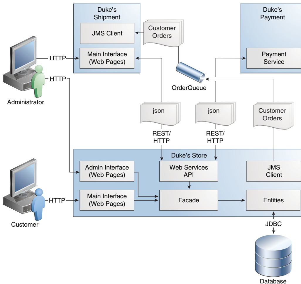
Figure 59–2 Interactions between Duke's Forest Components
