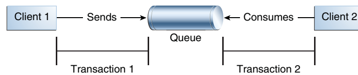
Figure 45–8 Using JMS Local Transactions
