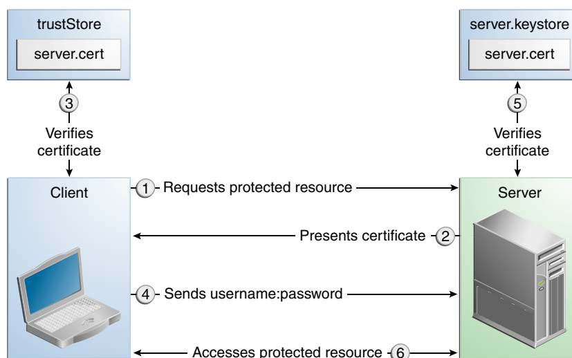
Figure 50-2 User Name/Password-Based Mutual Authentication
