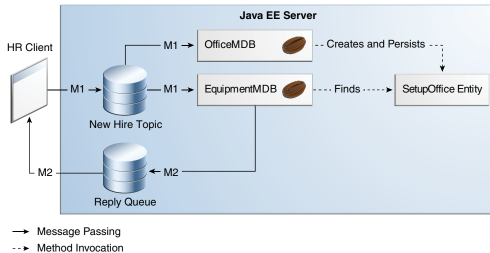
Figure 46-5 An Enterprise Bean Application: Client to Message-Driven Beans to Entity
