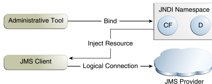
Figure 45–2 JMS API Architecture
