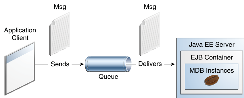
Figure 46–3 The simplemessage Application
