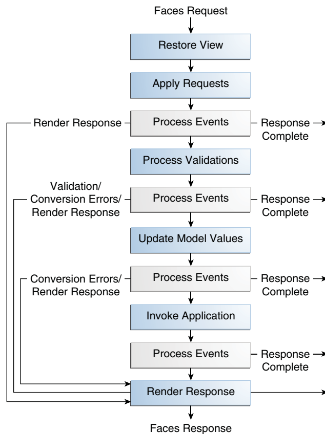
Figure 7-3 JavaServer Faces Standard Request-Response Lifecycle
