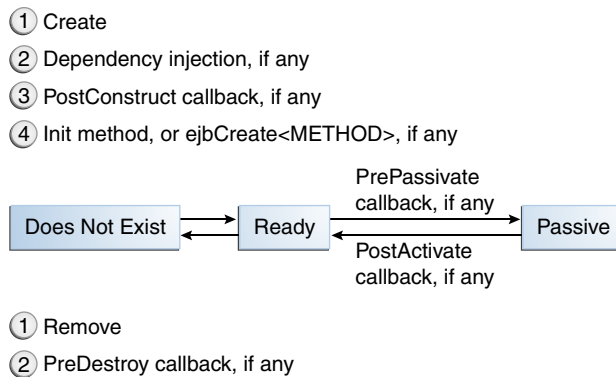
Figure 32–2 Lifecycle of a Stateful Session Bean
