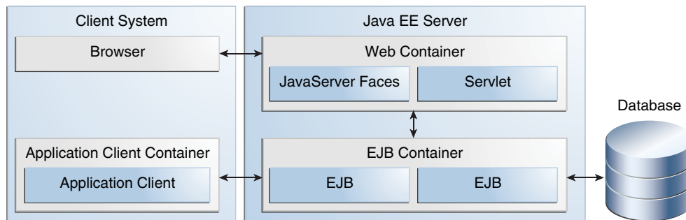
Figure 1–6 Java EE Containers
