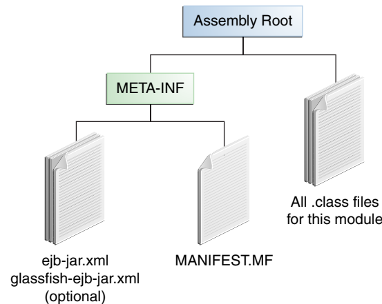
Figure 5-2 Structure of an Enterprise Bean JAR
