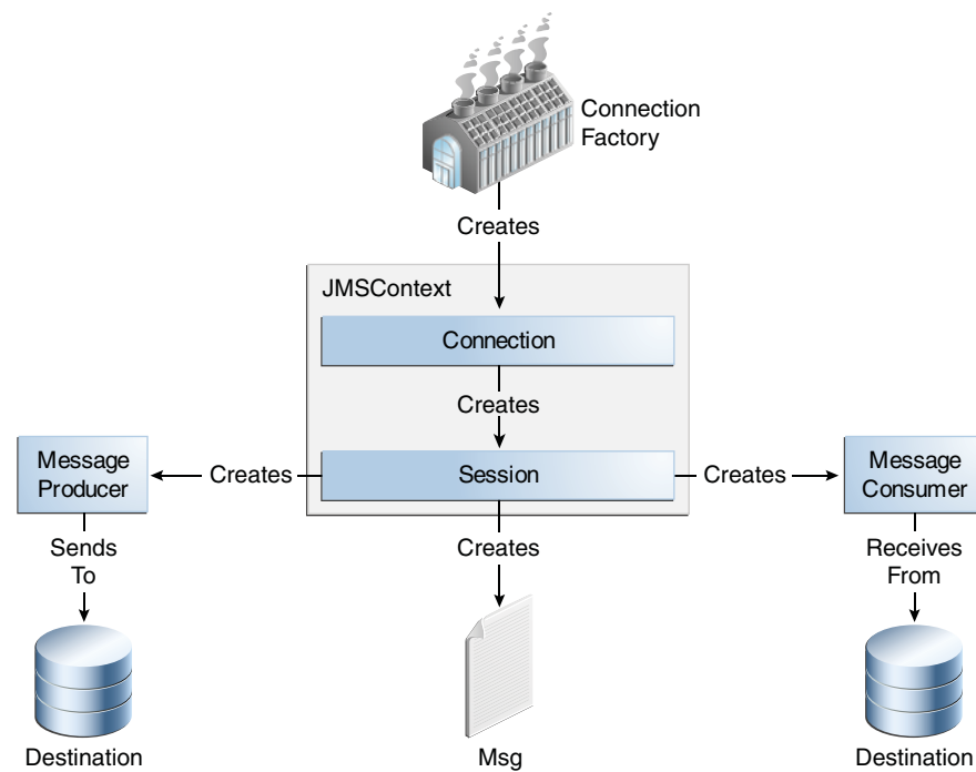
Figure 45-5 The JMS API Programming Model
