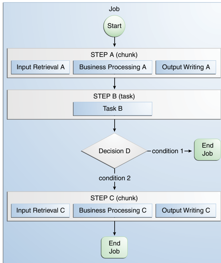
Figure 55–2 Steps and Decision Elements in a Job
