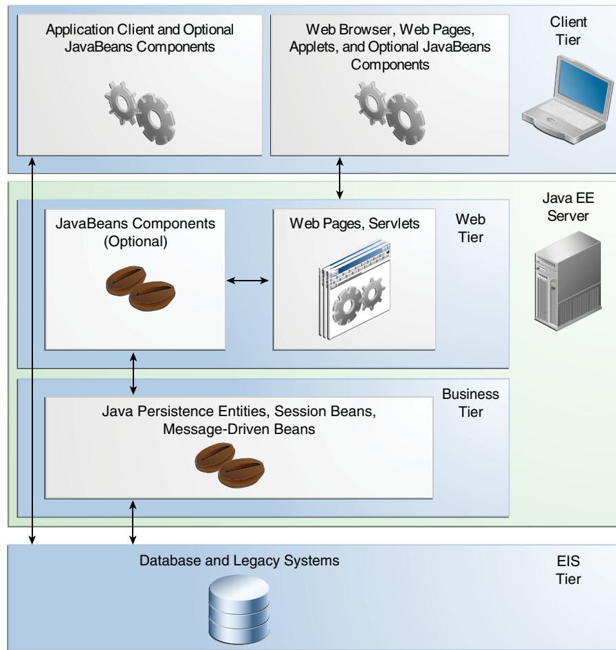
Figure 1–4 Business and EIS Tiers
