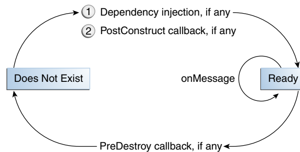
Figure 32-4 Lifecycle of a Message-Driven Bean
