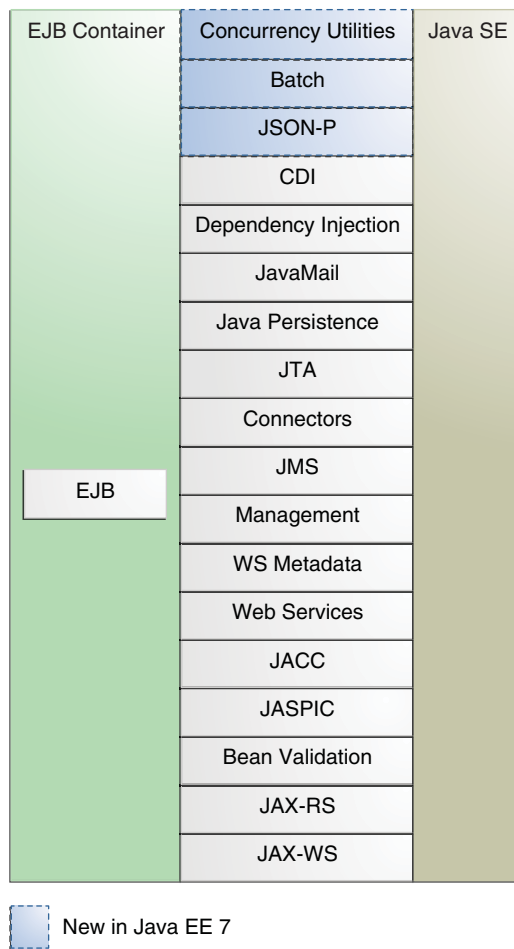
Figure 1–8 Java EE APIs in the EJB Container
