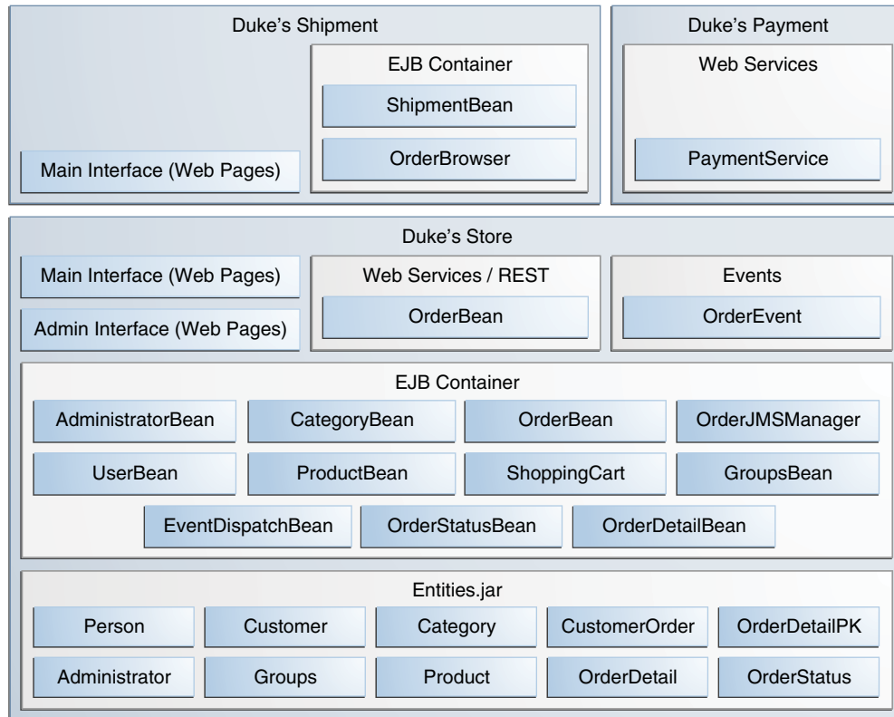
Figure 59–1 Architecture of the Duke's Forest Example Application
