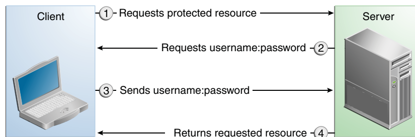
Figure 48–1 HTTP Basic Authentication
