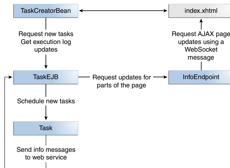
Figure 56–1 Architecture of the taskcreator Example
