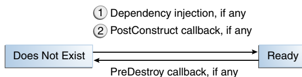
Figure 32–3 Lifecycle of a Stateless or Singleton Session Bean
