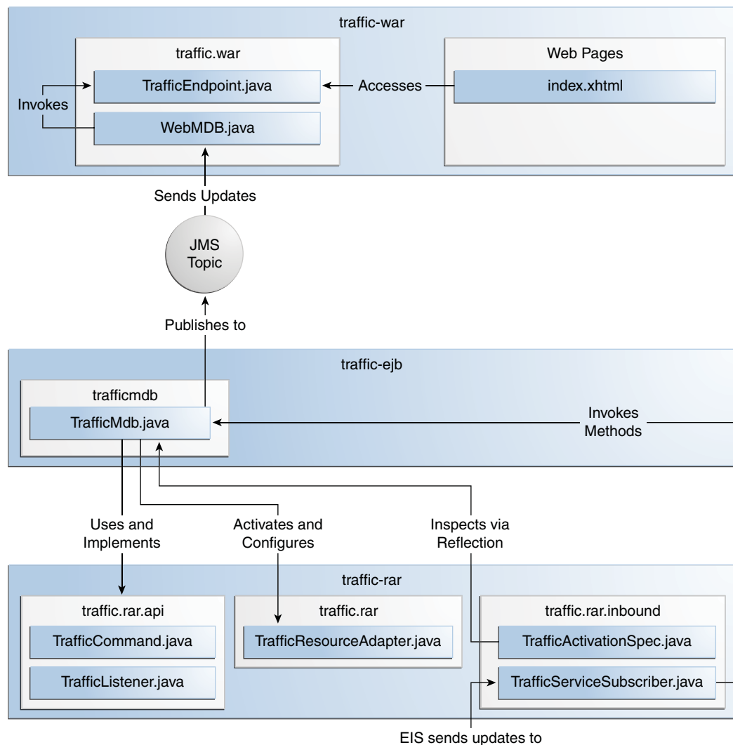
Figure 53–4 Architecture of the traffic Example
