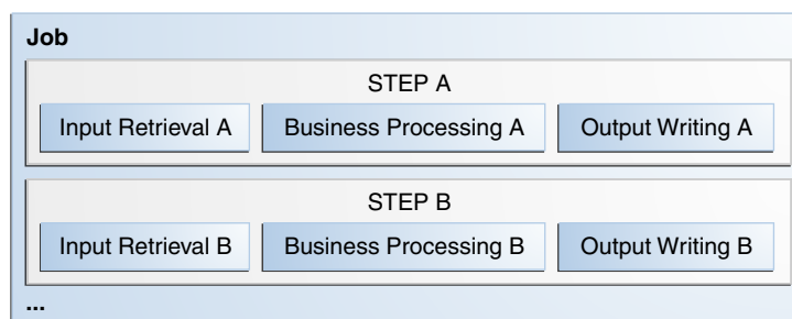
Figure 55–1 Chunk Steps in a Batch Job
