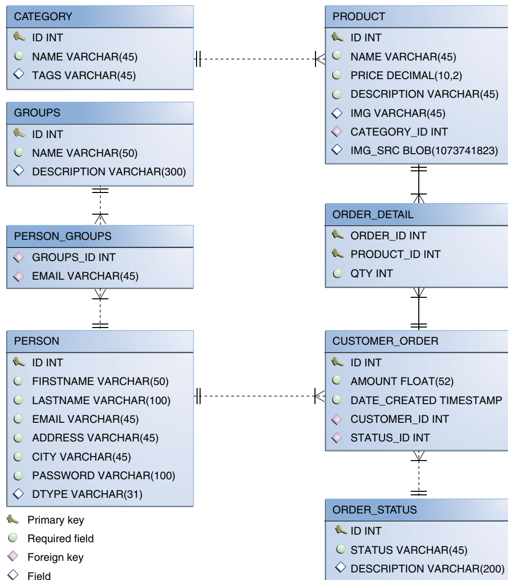
Figure 59-3 Duke's Forest Database Tables and Their Relationships
