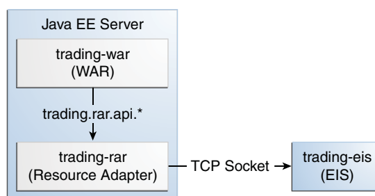
Figure 53–1 The trading Example
