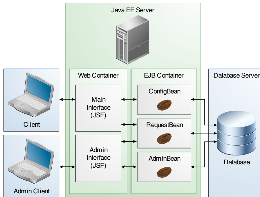
Figure 58–1 Architecture of the Duke's Tutoring Example Application
