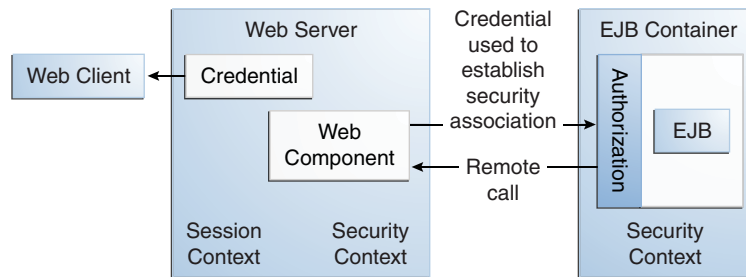
Figure 47-5 Invoking an Enterprise Bean Business Method
