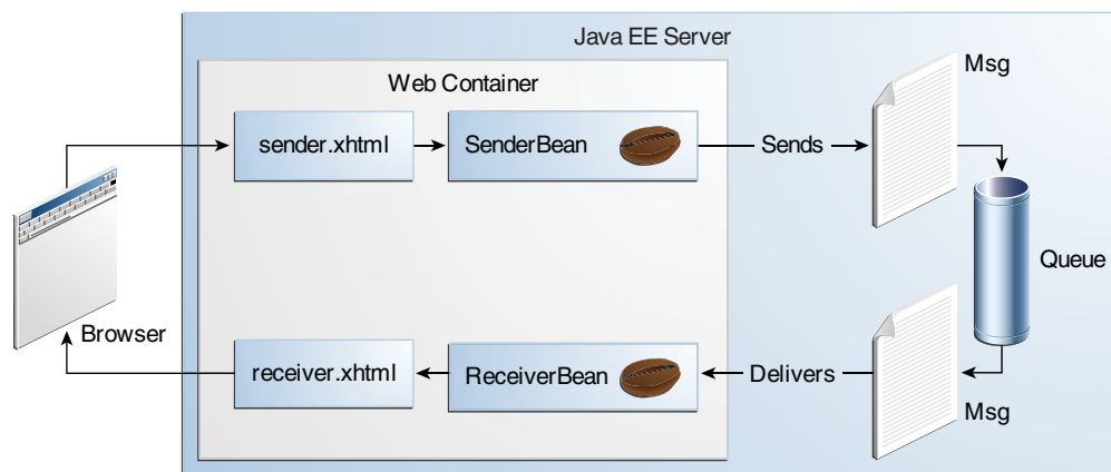
Figure 46–2 The websimplemessage Application
