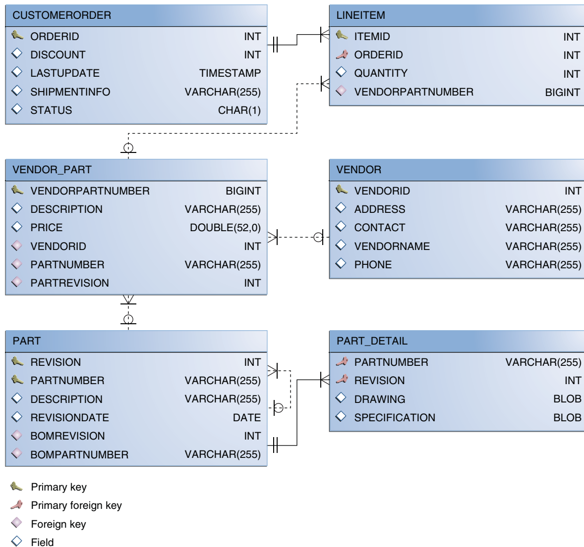
Figure 38–1 Database Schema for the order Application
