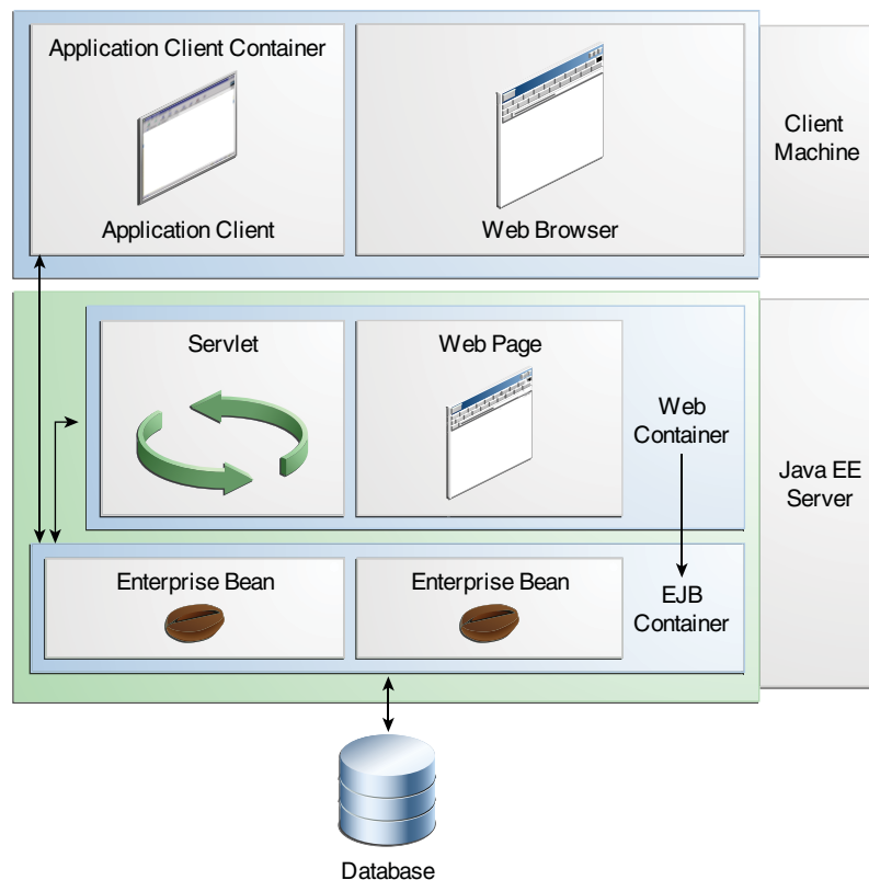
Figure 1–5 Java EE Server and Containers
