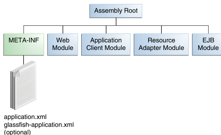
Figure 5–1 EAR File Structure
