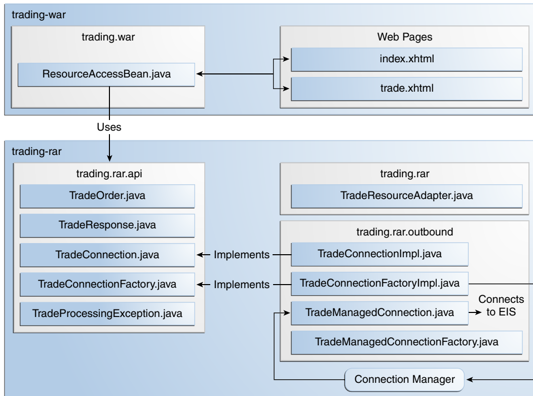
Figure 53-2 Architecture of the trading Example
