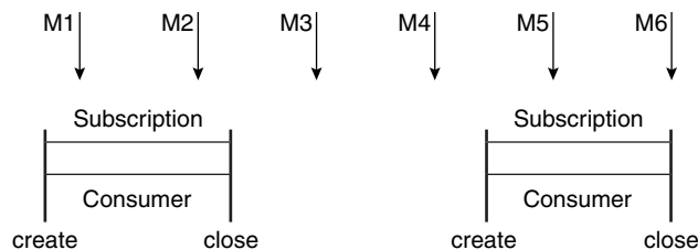
Figure 45–6 Nondurable Subscriptions and Consumers
