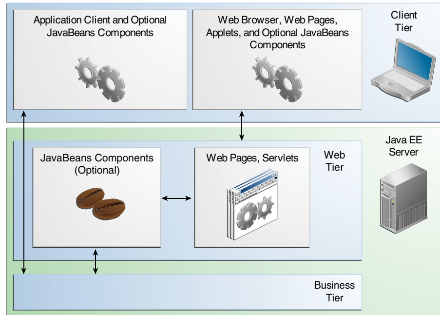
Figure 1-3 Web Tier and Java EE Applications
