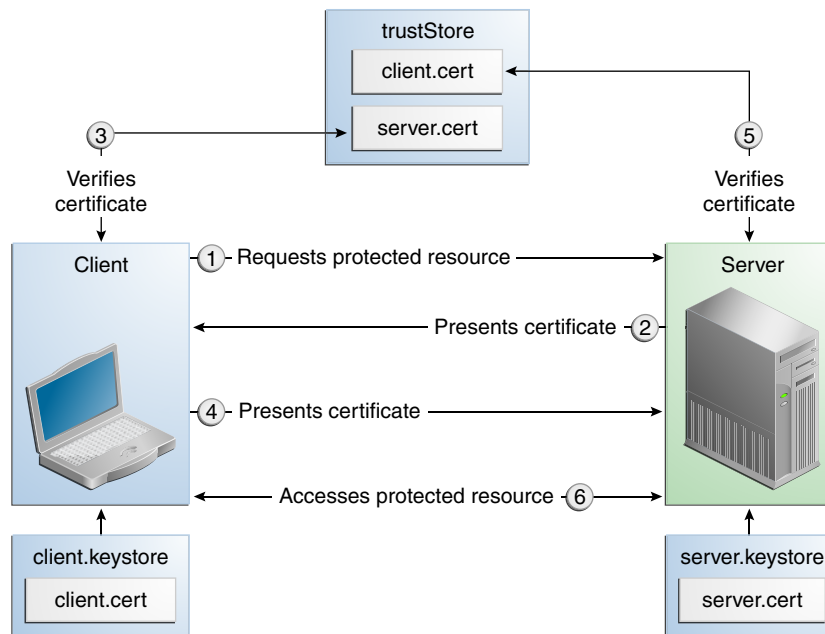
Figure 50–1 Certificate-Based Mutual Authentication
