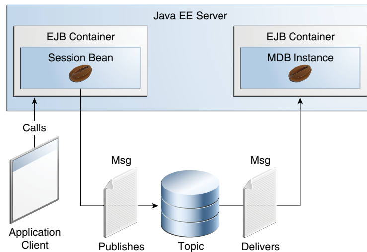
Figure 46–4 An Enterprise Bean Application: Client to Session Bean to Message-Driven Bean
