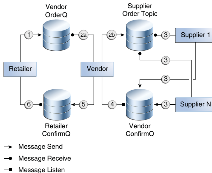
Figure 46–1 Transactions: JMS Client Example
