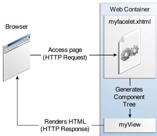
Figure 7-1 Responding to a Client Request for a JavaServer Faces Page
