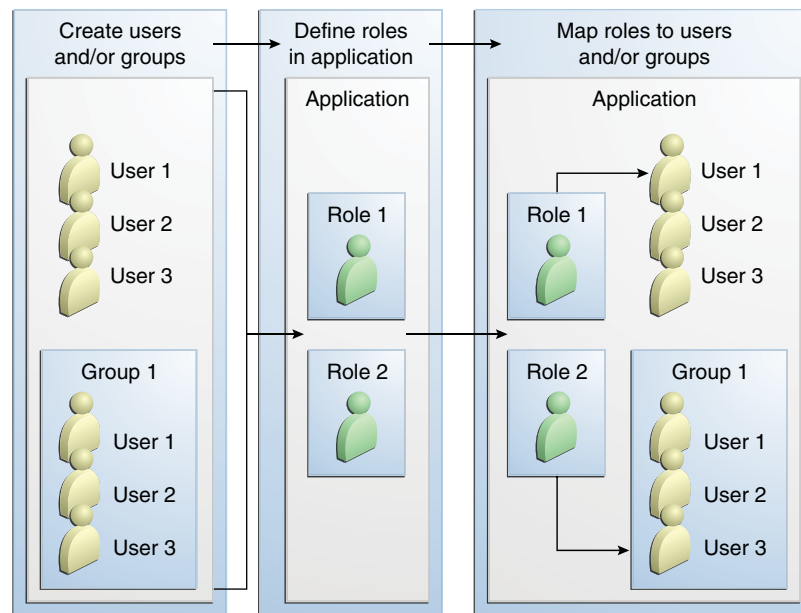
Figure 47-6 Mapping Roles to Users and Groups
