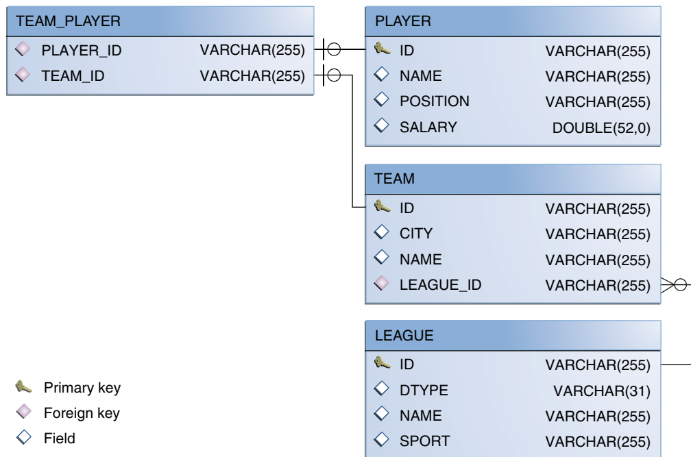
Figure 38–2 Database Schema for the roster Application
