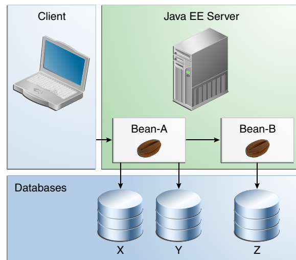
Figure 51–2 Updating Multiple Databases
