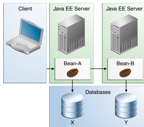
Figure 51–3 Updating Multiple Databases Across Java EE Servers
