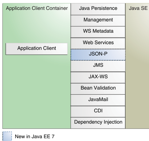
Figure 1–9 Java EE APIs in the Application Client Container
