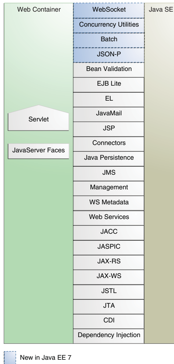
Figure 1–7 Java EE APIs in the Web Container
